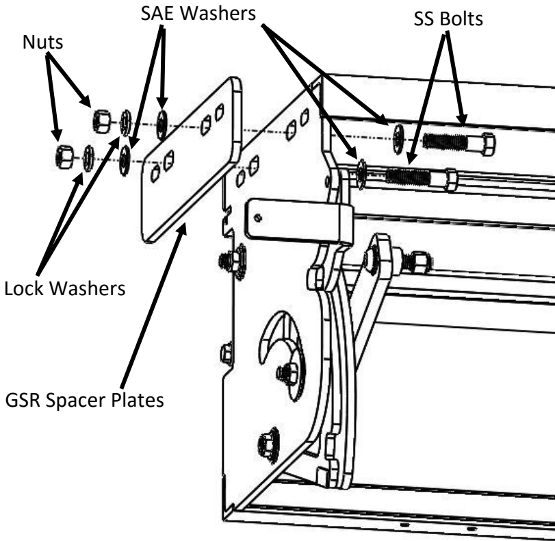
Figure 3.2 (3/8" hardware shown, when using 5/16" hardware use the 5/16 holes shown in Figure 4.1)
